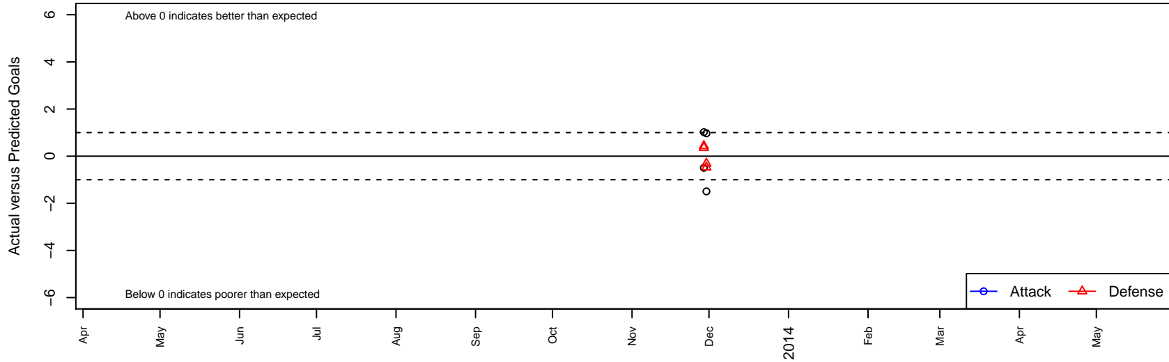
Impact Black B98 Dots are actual minus expected GF (blue circles) and GA (red triangles). Blue line is smoothed change in attack strength. Red is smoothed change in defense strength.
